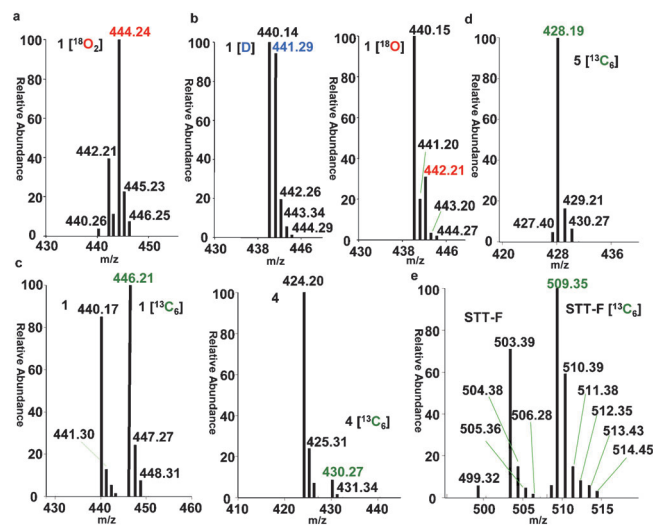
Figure 3. Mass spectrometric analyses. a) Spectrum of ^{18}\text{O}_2 -1. The product was obtained from the OrfP reaction conducted under ^{18}\text{O}_2 . b) Spectra of isotope-enriched 1. The reactions were performed using OrfP E15A in either a \text{D}_2\text{O} or \text{H}_2^{18}\text{O} buffer solution containing 1. c) Spectra of 1 and 4. In terms of yield, the labeled one is greater and less than the unlabeled for 1 (left) and 4 (right), respectively. d) Spectrum of ^{13}\text{C}_6 -5. e) Spectrum of STT-F extracted from the feeding experiment.
