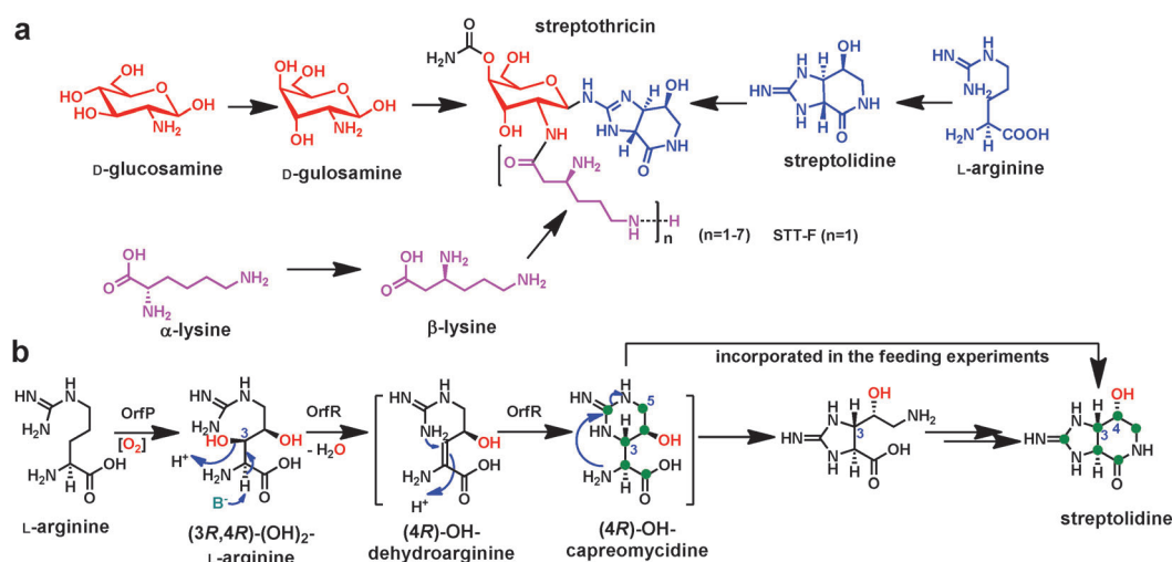
Figure 1. a) Chemical structures and biosynthesis of STT-F. b) Proposed enzyme reactions and feeding results for biosynthesis of streptolidine described in this study (green round dots stand for ^{13}\text{C} enrichment).
